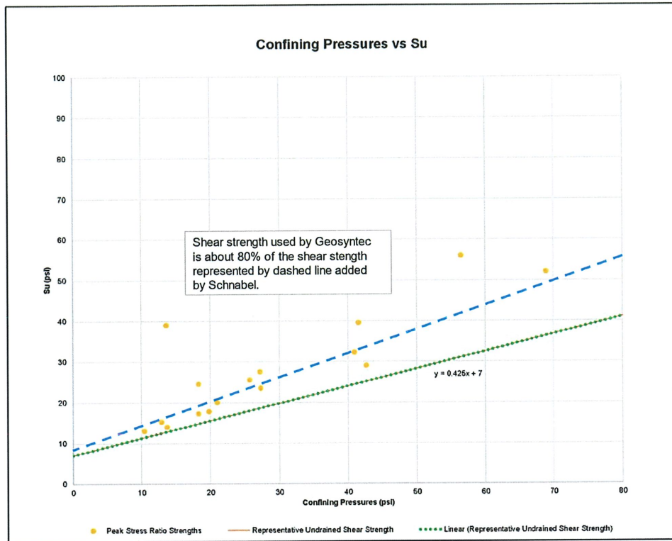
Figure 3: Undrained Shear Strength Characterization
